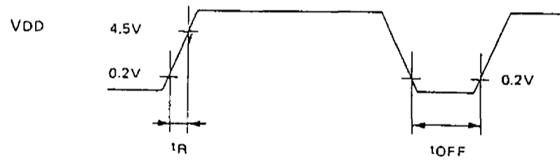
Fig. 9 Power on reset
