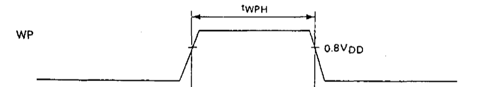
Fig. 8 Wake-up input timing
