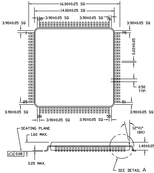
Figure 16. 100-pin TQFP (14 × 14 × 1.4 mm) A100SA Package Outline, 51-85048
