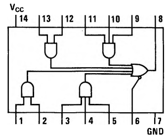
DM74H62
