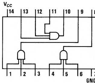
DM74H61
