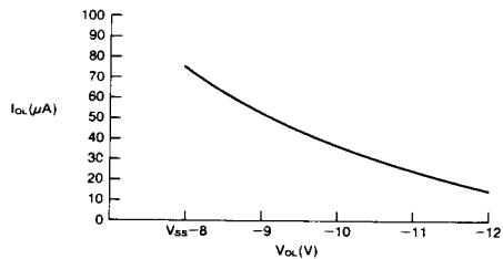
Fig.9 TYPICAL OUTPUT SINK CURRENT vs OUTPUT VOLTAGE
