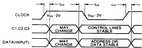
Fig.7 INPUT TIMING
