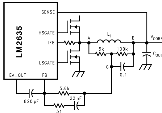
Figure 8. Dynamic Voltage Positioning by Utilizing Output Inductor DC Resistance
