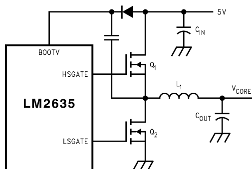
Figure 4. BOOTV Voltage Supplied by a Charge Pump
