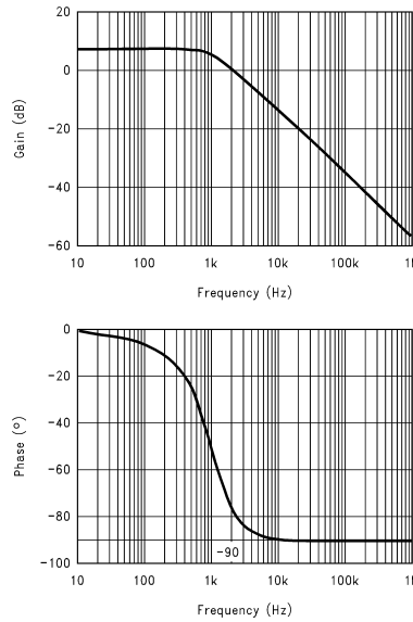
Figure 6. Control-to-Output Bode Plots
