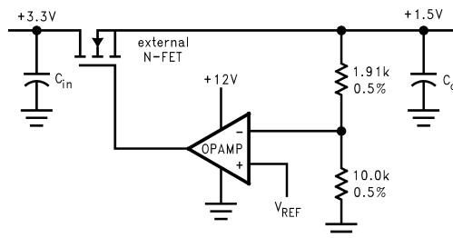
Figure 10. V_{REF} Used in an N-FET LDO Supply
