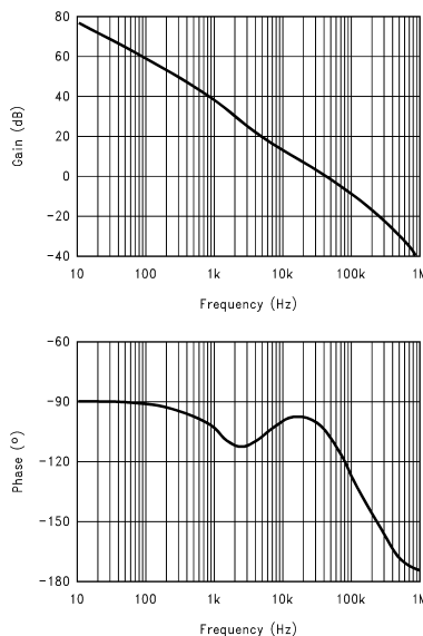
Figure 7. Loop Bode Plots
