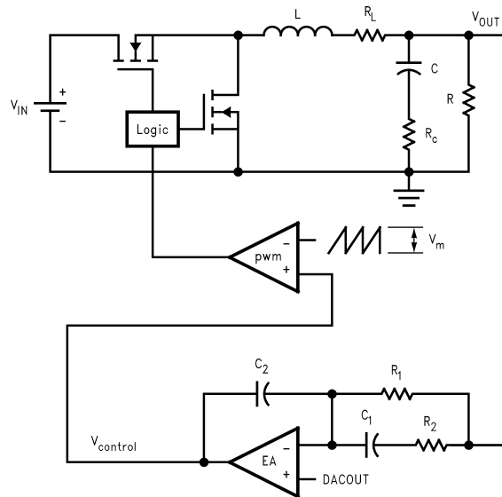
Figure 5. Buck Converter from a Control Point of View
