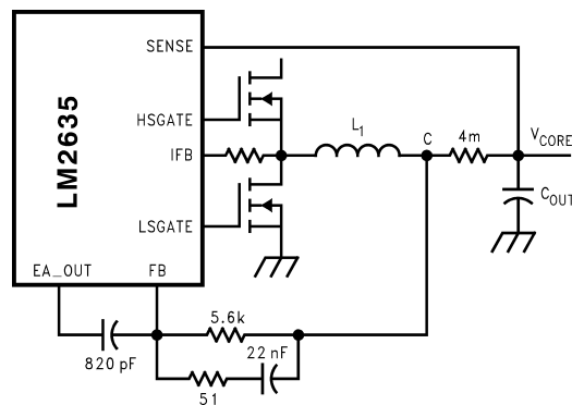
Figure 9. Dynamic Voltage Positioning by Using A Stand-Alone Resistor
