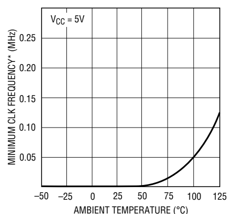
Minimum Clock Rate for 0.1 LSB Error
