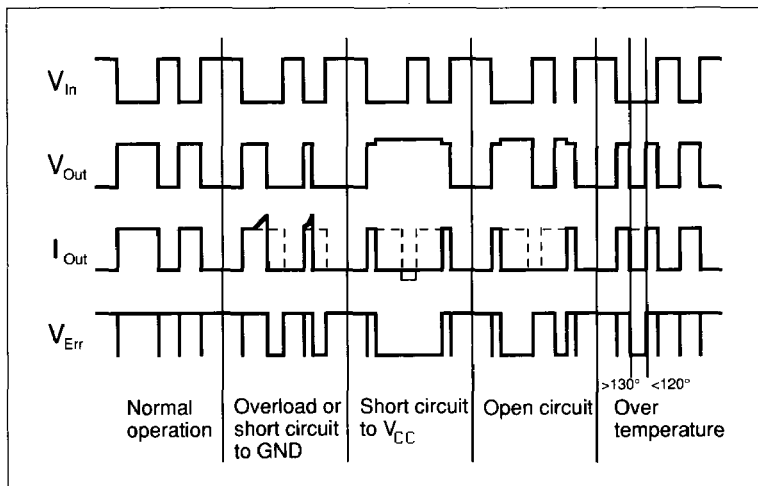
Figure 18. Signal diagram
