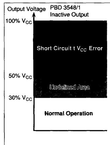
Figure 6. Error state vs. output voltage, inactive output ( 2.0V \leq V_{IN} \leq V_{CC} , 5V \leq V_{CC} \leq 40V and -40^\circ C < T_J < +100^\circ C ).
