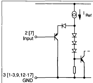
Figure 15. Input stage.
