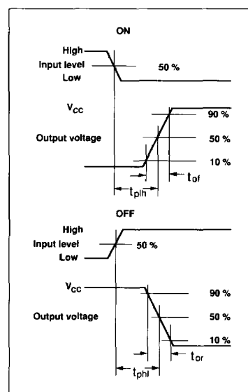
Figure 3. Timing diagram, input vs. output. V_{CC} = 24V .
