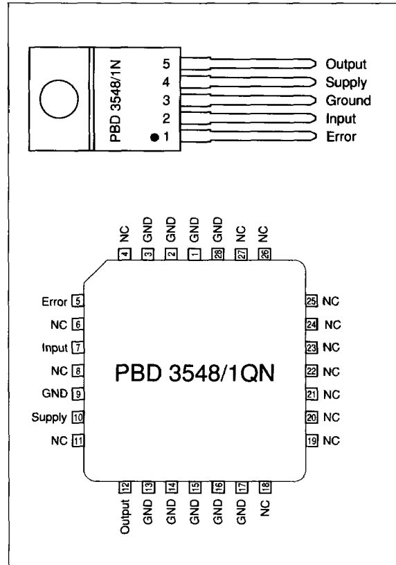
Figure 4. Pin descriptions.
