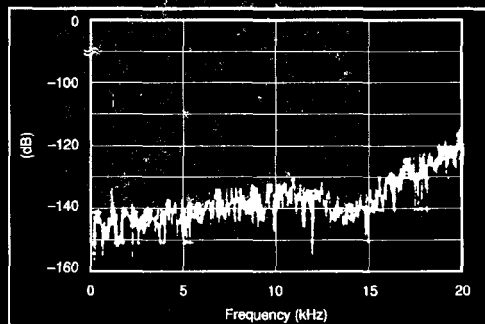
FIGURE 3. Quantization Noise Spectrum (256fs).
