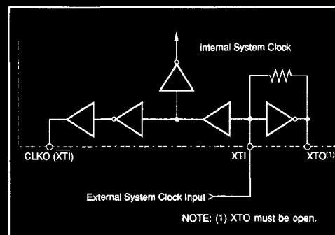
FIGURE 10. Oscillator Circuit Connection Diagram. External system clock.
