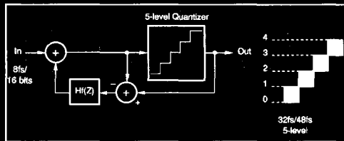
FIGURE 1. Block Diagram of 5-Level Delta-Sigma Quantizer.
