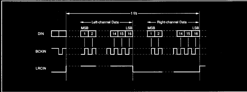
FIGURE 5. Data Input Timing, 16-Bit.
