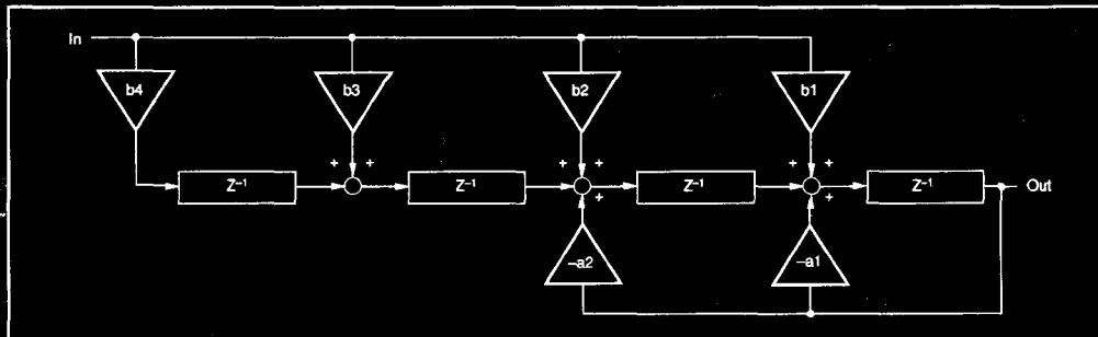
FIGURE 2. Block Diagram of the H_f(z) .
