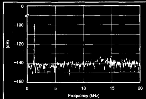
FIGURE 4. Quantization Noise Spectrum (384fs).
