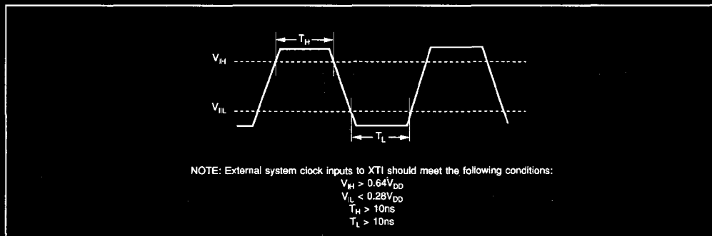
FIGURE 8. Operation Instruction For System Clock.
