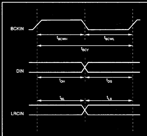
FIGURE 6. Data Input Timing.
