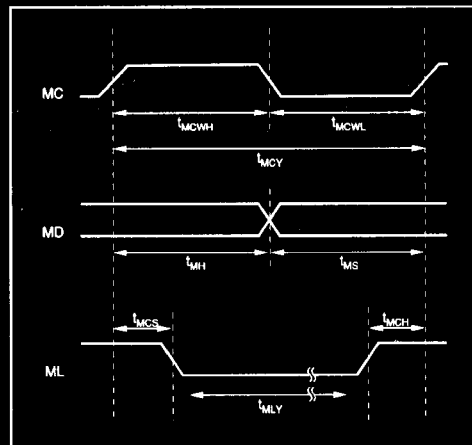
FIGURE 7. Serial Mode Control Timing.
