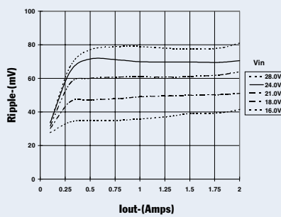
Ripple vs Output Current
