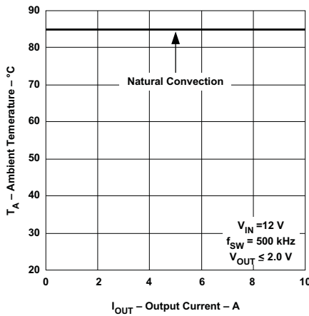
Figure 7. Safe Operating Area
