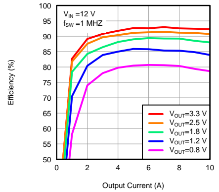
Figure 3. Efficiency
