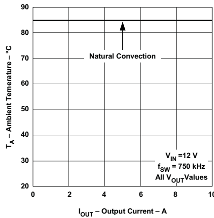
Figure 8. Safe Operating Area
