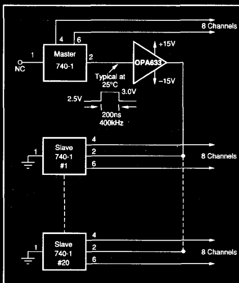
FIGURE 1. Master/Slave Synchronization of Multiple PWS740 Drivers.
