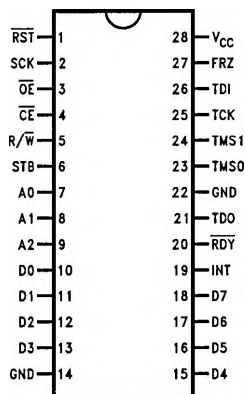
28-Pin SOIC, DIP and Flatpak
