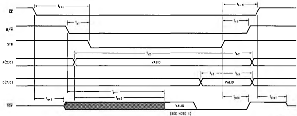
FIGURE 2. Write Cycle
