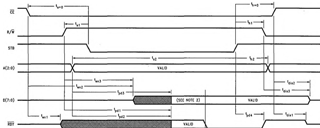
FIGURE 3. Read Cycle
