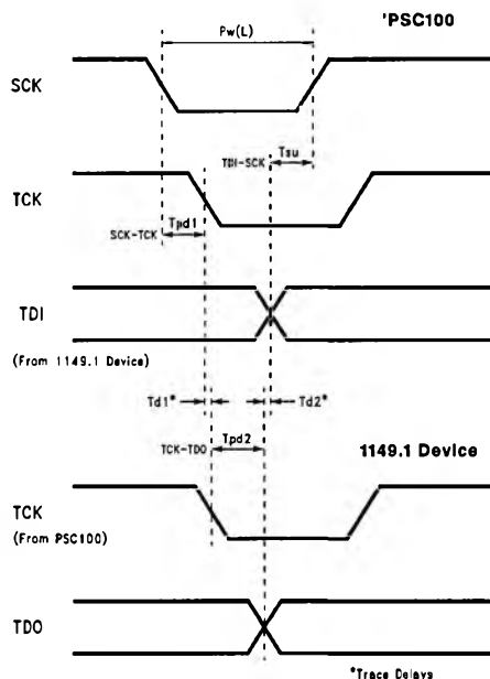
FIGURE 16. System Clock Timing for Accurate TDI Data
