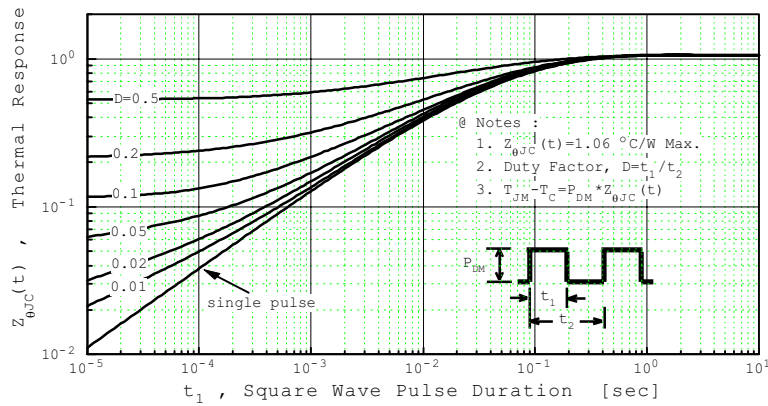
Fig 11. Thermal Response
