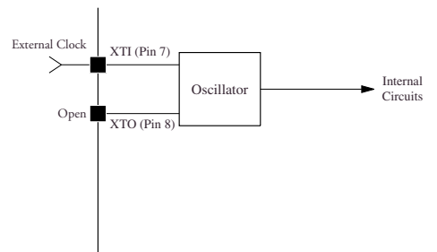
Figure 6. External clock input (SM8707J)
