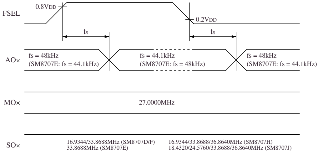
Figure 8. Output signal switching timing
