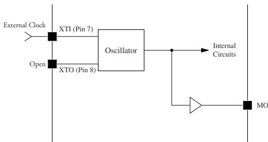
Figure 5. External clock input (excluding SM8707J)
