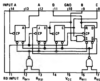
DM5490/DM7490
