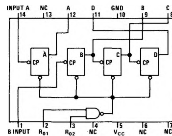
DM5493/DM7493
