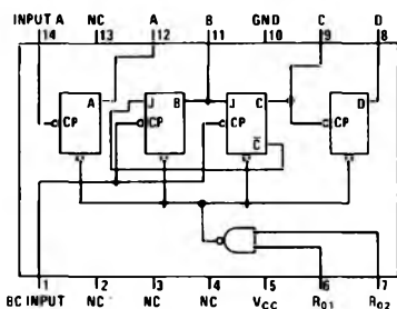
DM5492/DM7492
