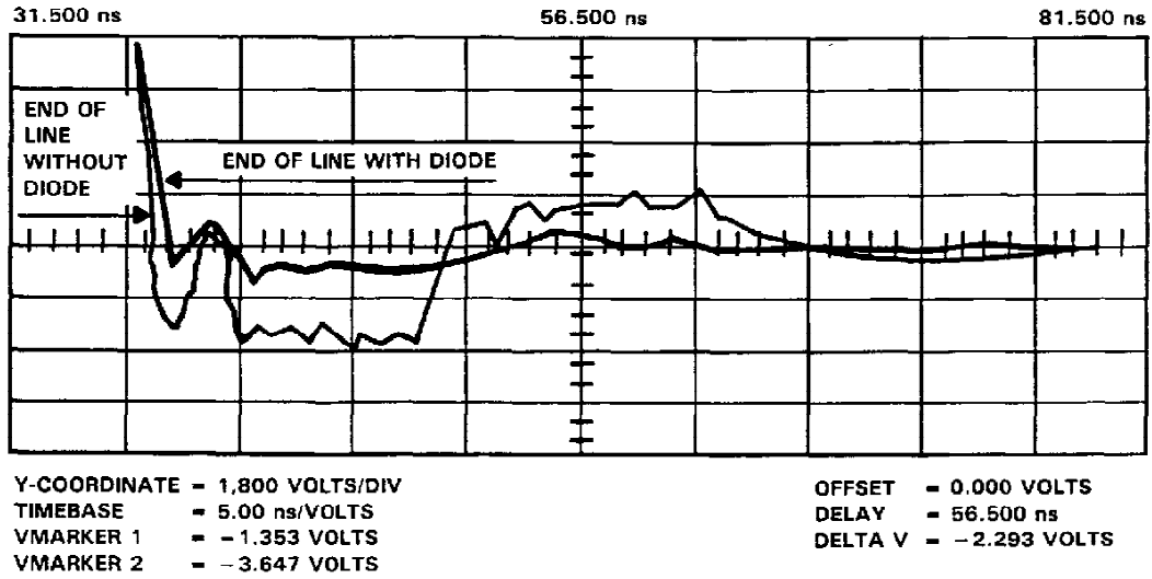
FIGURE 5. SCOPE DISPLAY
