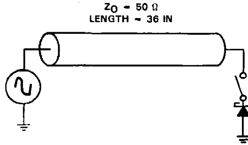
FIGURE 4. DIODE TEST SETUP
