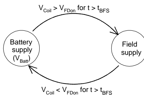
Figure 5. Switch conditions for the power management
