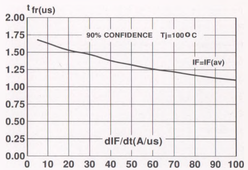
Fig.15 : Recovery time versus dIF/dt.
