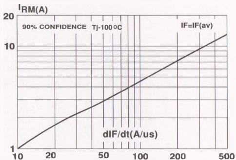
Fig.12 : Peak reverse current versus dIF/dt.
