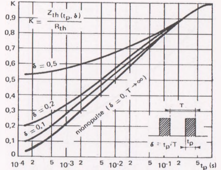
FIGURE 4 : Thermal impedance versus pulse width
