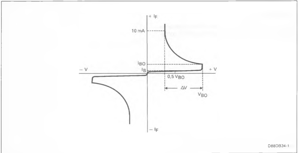
DIAGRAM 1 : Current-voltage characteristics.
