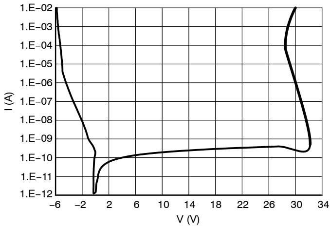
Figure 1. IV Characteristics
