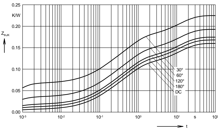
Fig. 9 Transient thermal impedance junction to heatsink (per diode)
