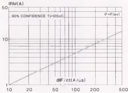
Fig.9 : Peak reverse current versus dI/dt . (Per diode)
