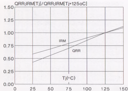
Fig.13 : Dynamic parameters versus junction temperature.
