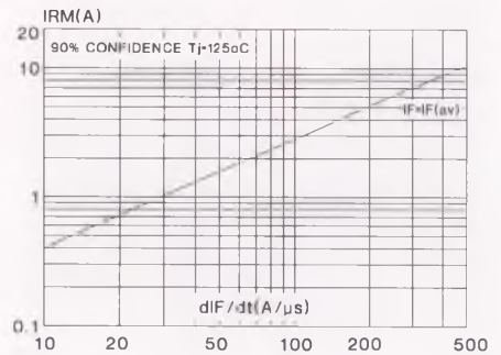
Fig.12 : Peak reverse current versus dI/dt . (Per diode)
