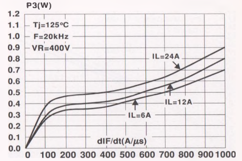
Fig 6 : Switching OFF losses versus dI/dt
