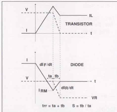
Fig. 4: TURN-ON CHARACTERISTICS
