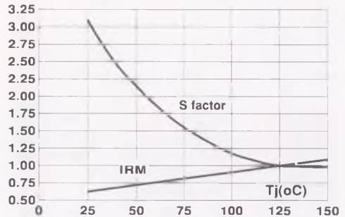
Fig 14 : Relative variation of dynamic parameters versus junction temperature (Reference Tj=125°C)
