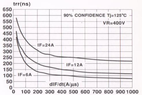
Fig 14 : Reverse recovery time versus dI_F/dt
