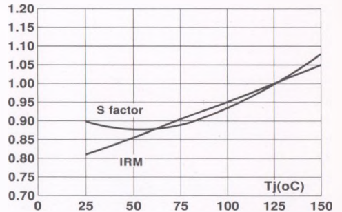
Fig 16 : Relative variation of dynamic parameters versus junction temperature (Reference T_j=125^\circ\text{C} )
