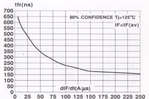
Fig 18 : Forward recovery time versus dI_F/dt
