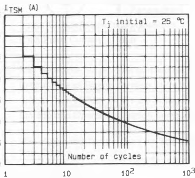
Fig.4 - Non repetitive surge peak on-state current versus number of cycles.
