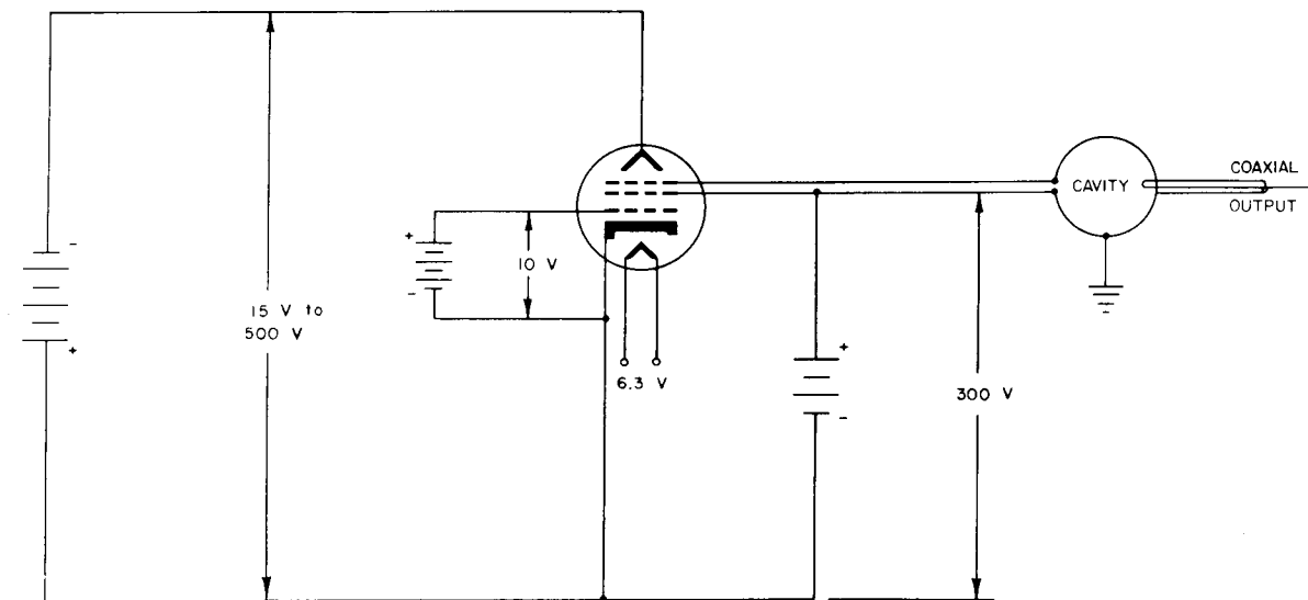
FIG. 1 — CW OSCILLATOR CIRCUIT EMPLOYING THE 5837 REFLEX KLYSTRON
