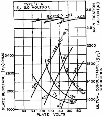
AVERAGE CHARACTERISTICS
