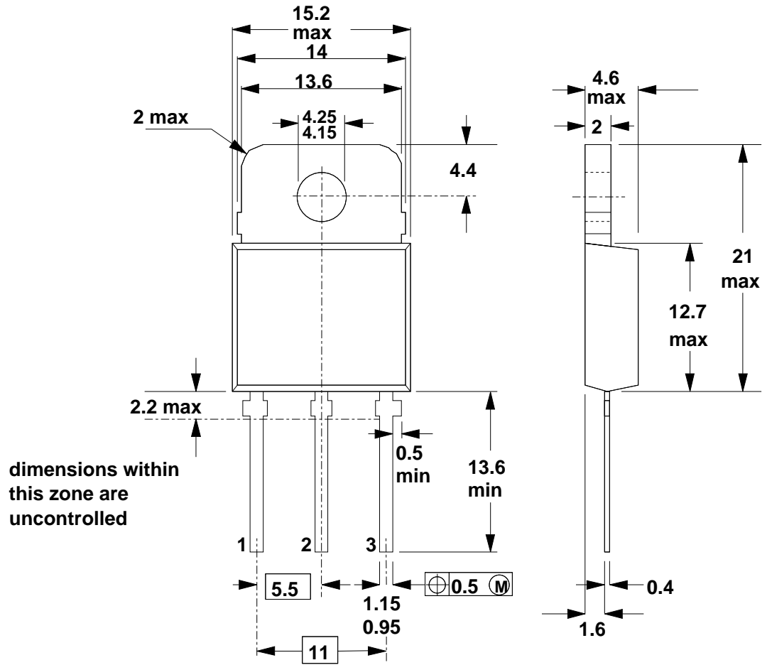
Fig.16. SOT93; pin 2 connected to mounting base.
