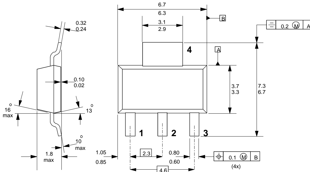
Fig.20. SOT223 surface mounting package 1 .
