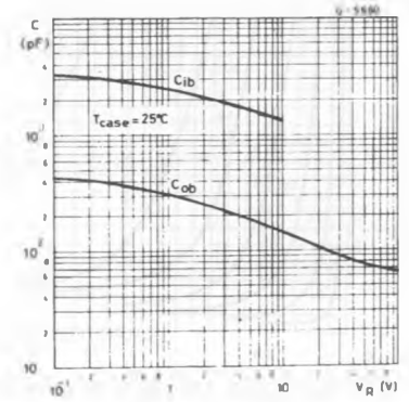
Capacitance.
