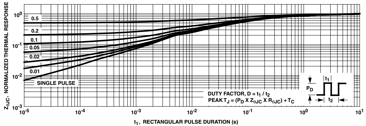
FIGURE 16. NORMALIZED TRANSIENT THERMAL RESPONSE, JUNCTION TO CASE
