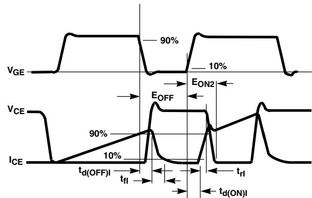
FIGURE 18. SWITCHING TEST WAVEFORMS
