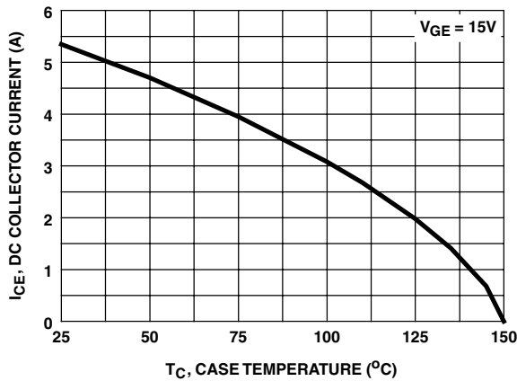
FIGURE 1. DC COLLECTOR CURRENT vs CASE TEMPERATURE
