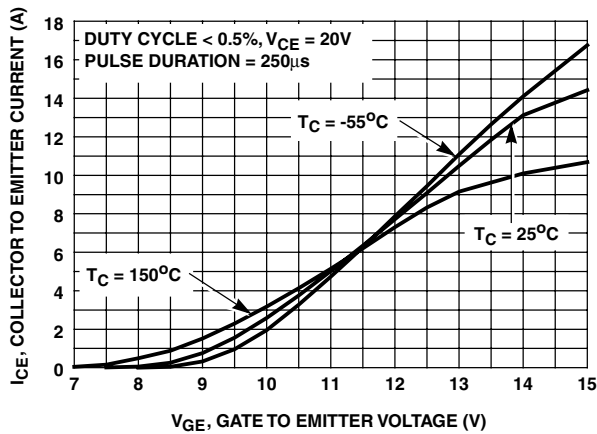
FIGURE 13. TRANSFER CHARACTERISTIC
