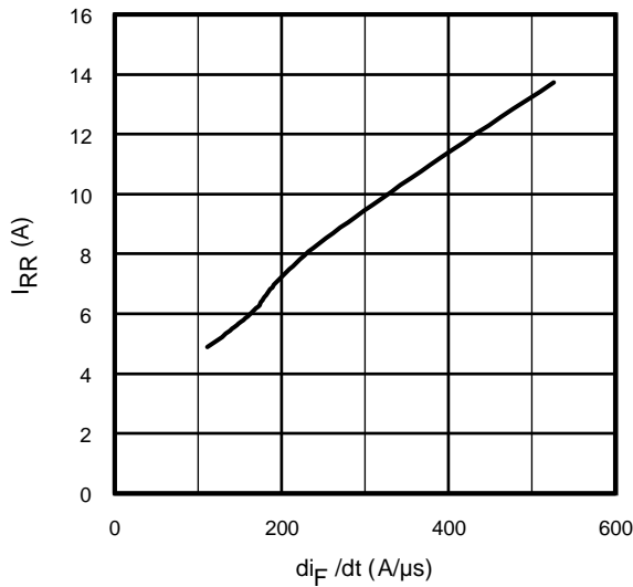
Fig. 19 - Typical Diode I_{RR} vs. di/dt V_{CC} = 400\text{V} ; V_{GE} = 15\text{V} ; I_{CE} = 10\text{A} ; T_J = 150^\circ\text{C}
