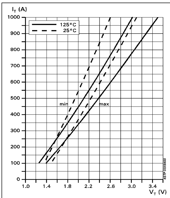
Fig. 2 On-state characteristics.
