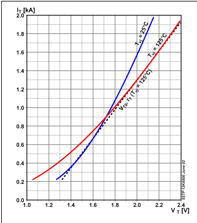
Fig. 2 Isothermal on-state characteristics
