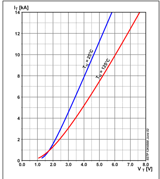
Fig. 3 Isothermal on-state characteristics
