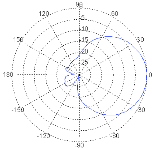
Elevation (E-field) radiation pattern
