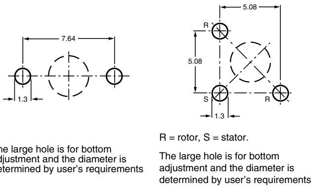
Hole pattern
