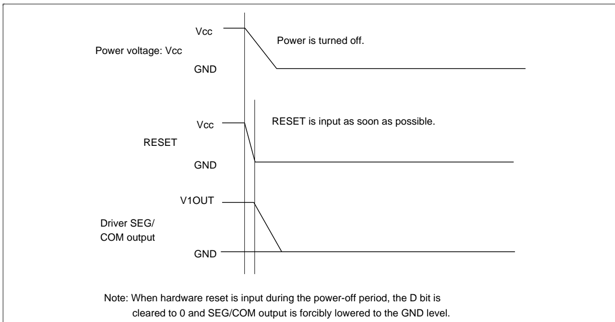
Figure 59 Power-off Timing
