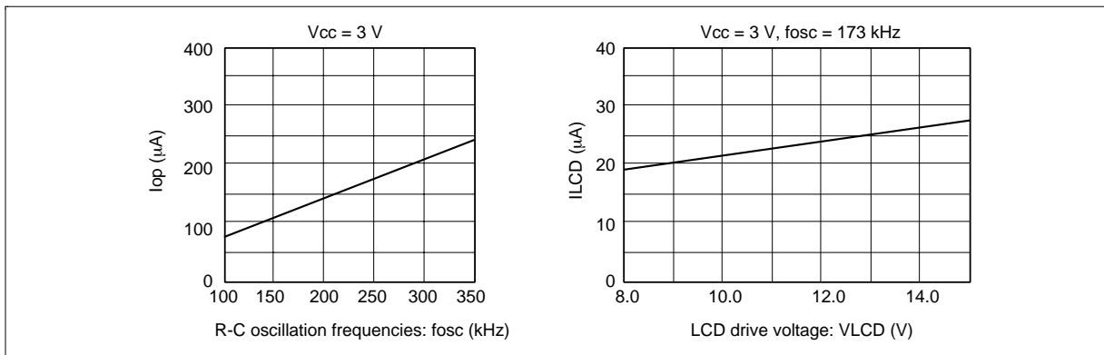
Figure 61 Relationship between the Operation Frequency and Current Consumption
