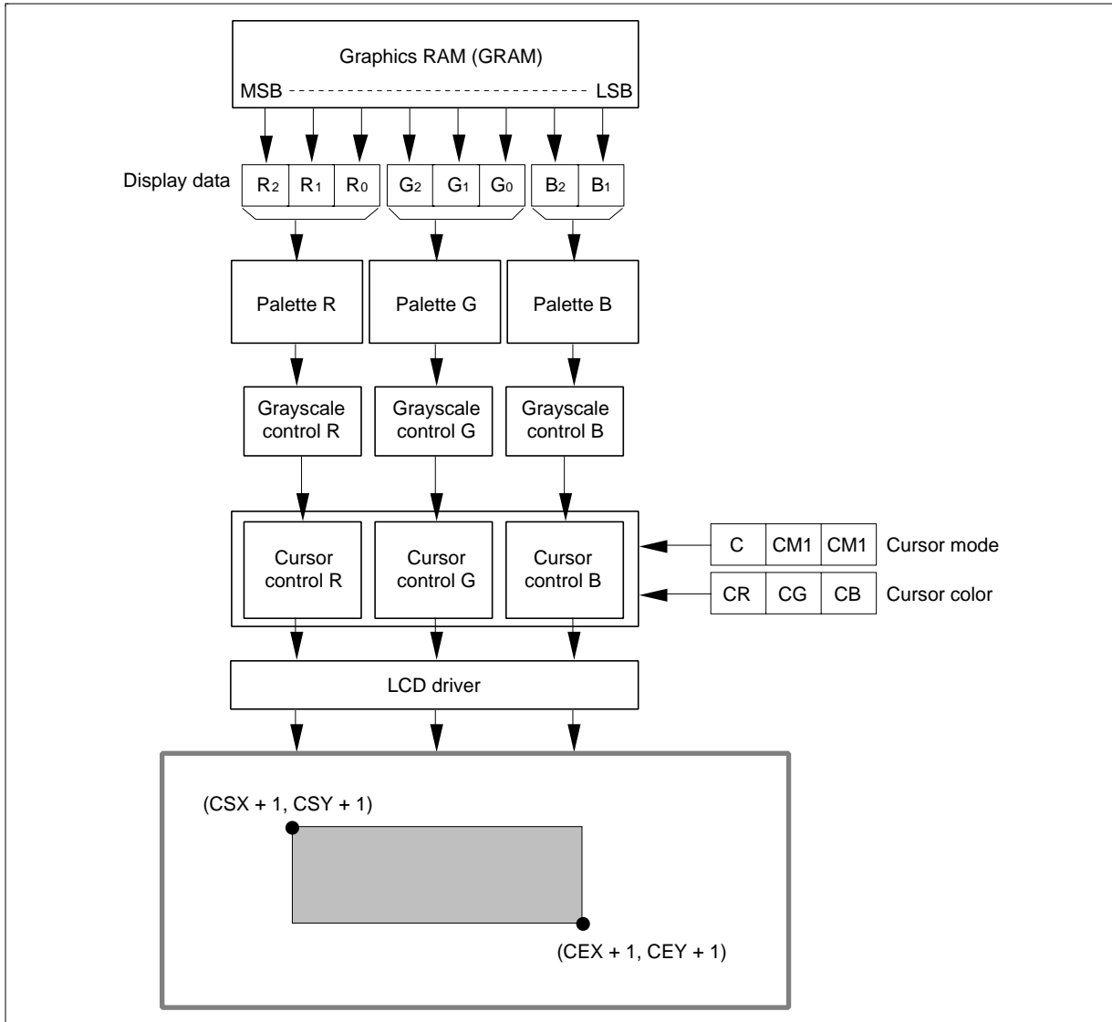
Figure 44 Color-cursor Display
