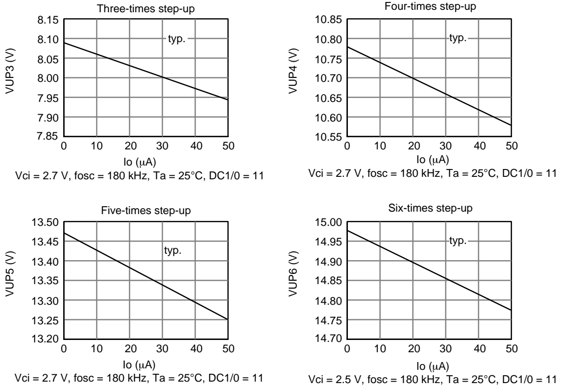
Figure 65 Step-up (cont)
