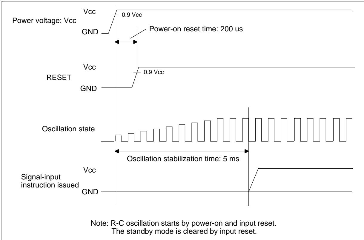
Figure 57 Power-on Timing
