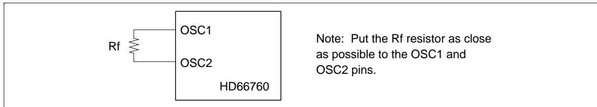
Figure 45 Oscillation Circuits
