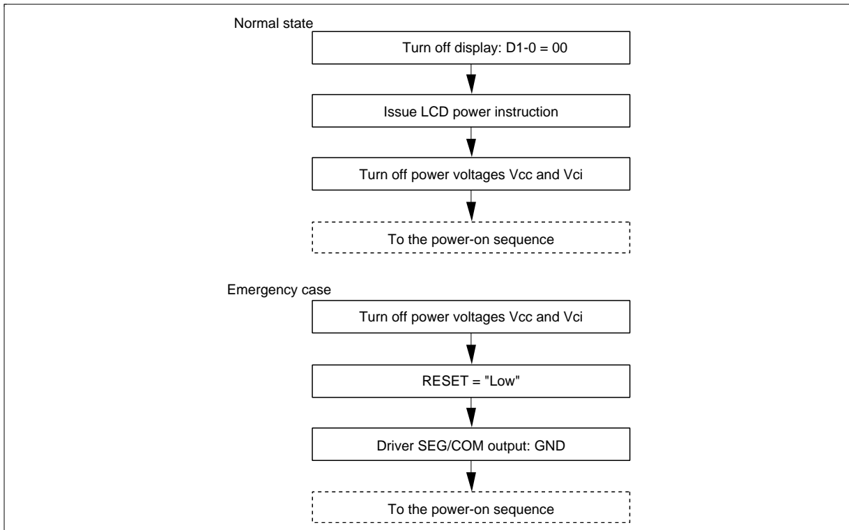
Figure 58 Power-off Sequence
