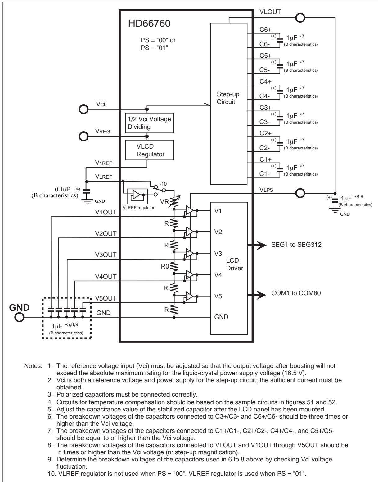
Figure 50 Internal Step-up Circuit for LCD Drive Voltage Generation
