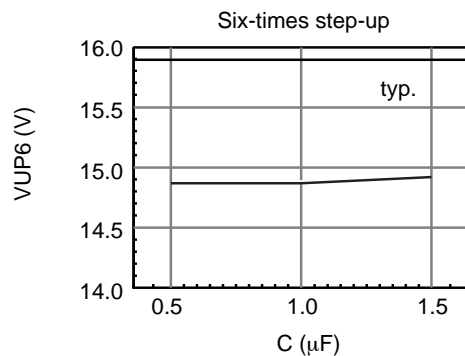
Figure 65 Step-up (cont)
