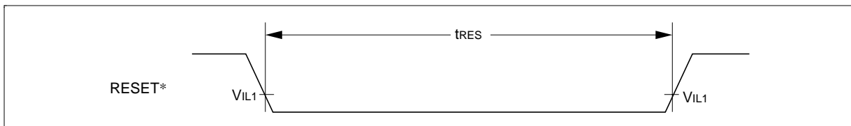
Figure 69 Reset Timing
