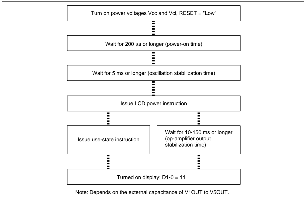
Figure 56 Power-on Sequence
