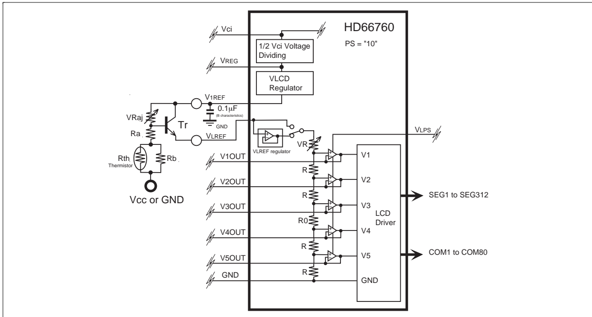
Figure 52 Temperature Compensation Circuits (2)
