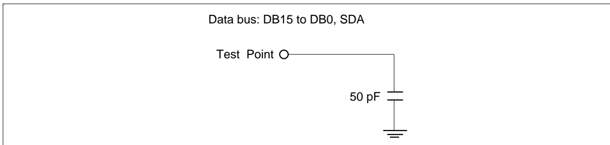
Figure 66 Load Circuit
