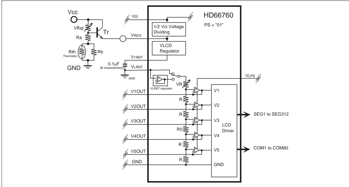
Figure 51 Temperature Compensation Circuits (1)
