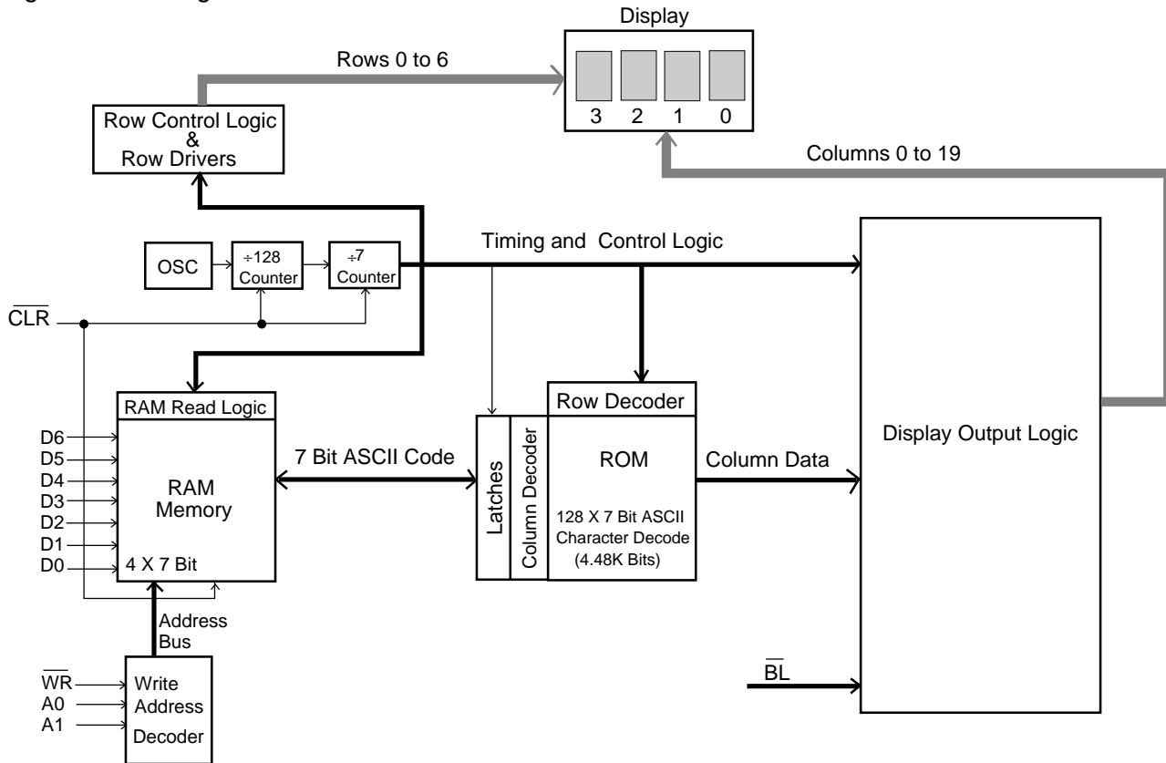
Figure 6. Block diagram
