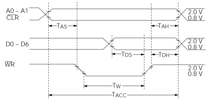
Figure 2. Timing characteristics—write cycle waveforms
